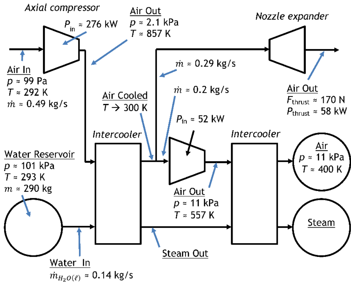
Figure 10. Compressor schematic for passenger capsule.
